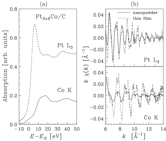
FIG. 3. (a) Comparison of Pt L_3 and Co K near-edge XAS spectra of \text{Pt}_{3\pm\delta}\text{Co} -Vulcan powder. E_0 is the edge energy. (b) Experimental \chi(k) signals of \text{Pt}_{3\pm\delta}\text{Co} -Vulcan nanopowder and \text{Pt}_{3\pm\delta}\text{Co} thin film. Top panel shows Pt L_3 edge, bottom panel shows Co K edge.
