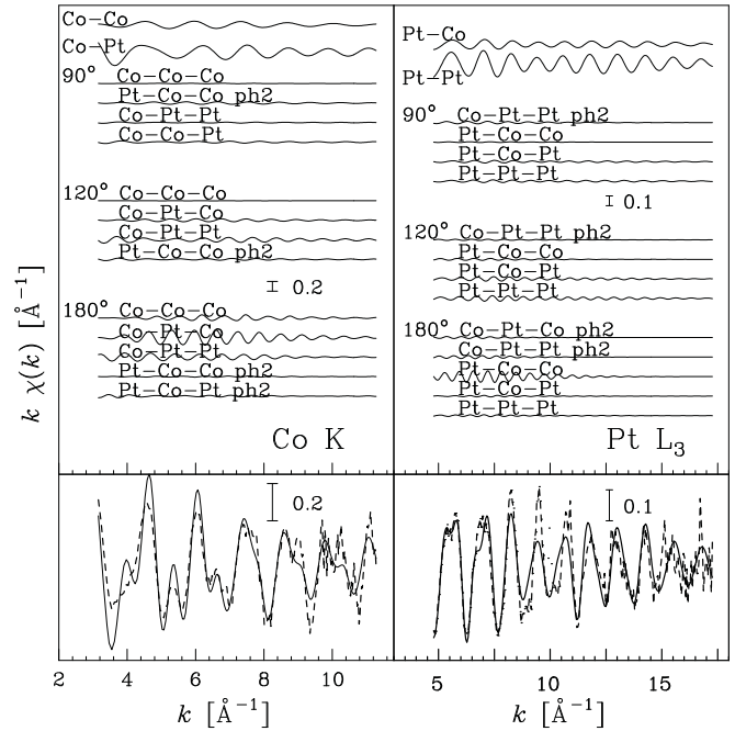
FIG. 8. The best double-edge-fit results of a GNXAS analysis performed for \text{Pt}_{3\pm\delta}\text{Co} thin film at Co K edge (left) and Pt L_3 edge (right). Upper curves represent components of the model signal, vertically shifted for clarity. The solid line is the model signal and the dashed line is the experimental signal. The scale is indicated within the figure.
